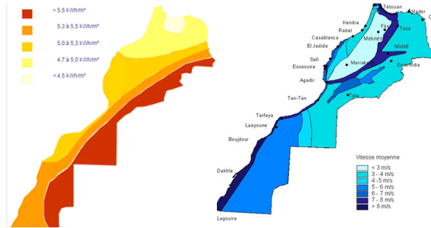
Solar and Wind energy map in Morocco
